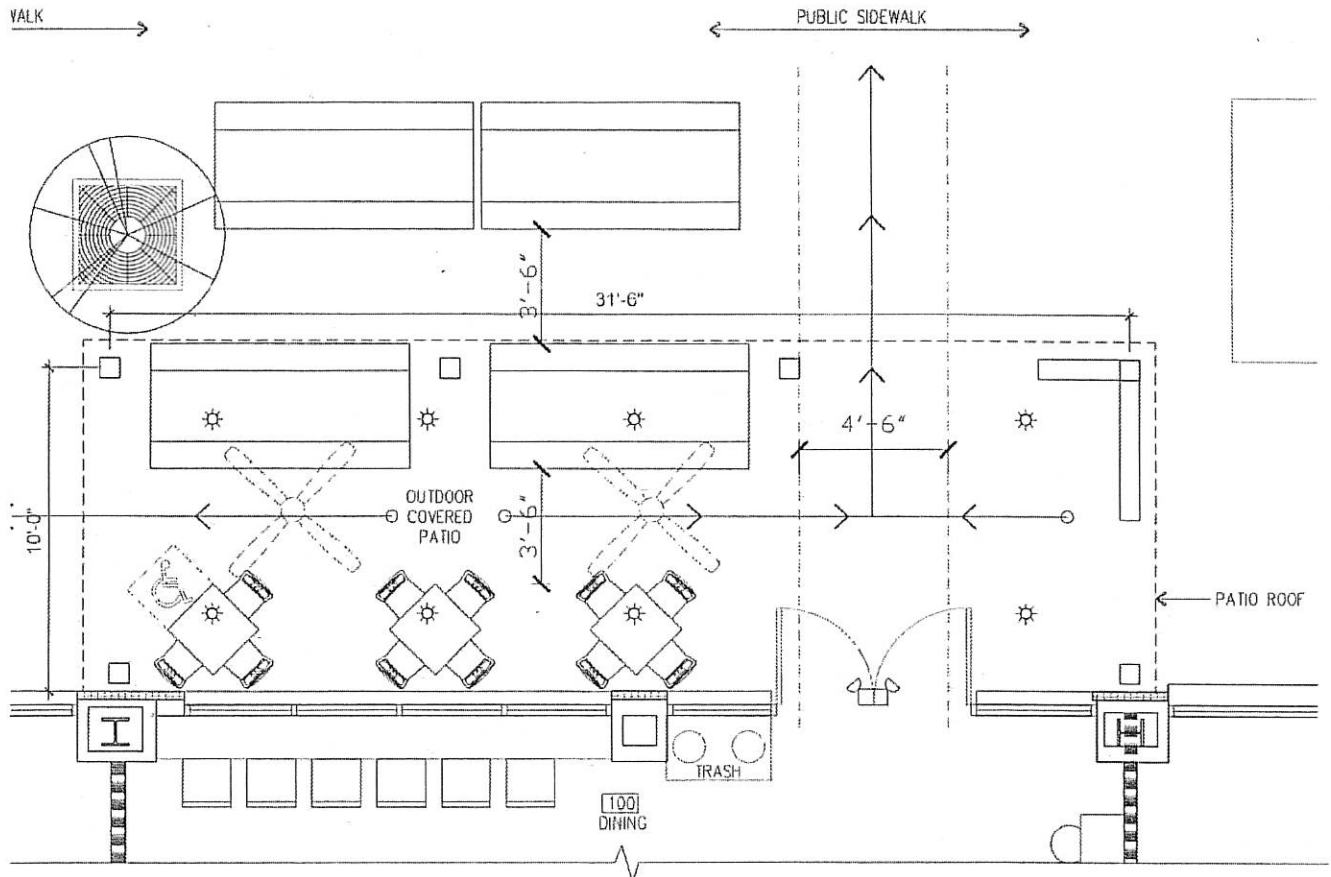
1 A1 OUTDOOR PATIO PLAN SCALE: 1/2" = 1'
