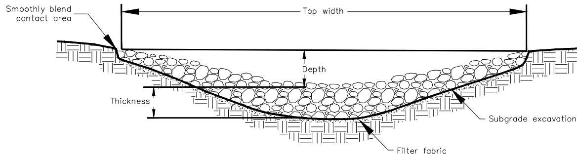
Parabolic-shaped Riprap Channel
