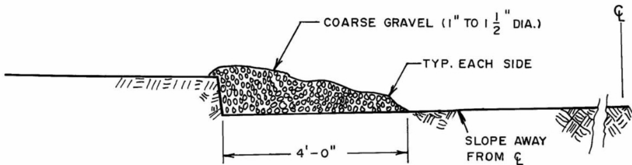
CHECK DAM
